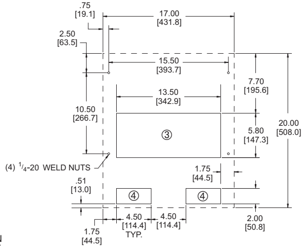
MOUNTING PLAN
