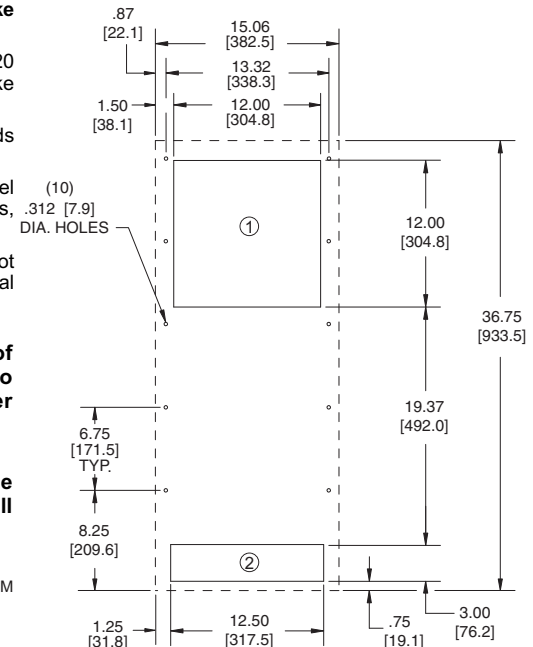
MOUNTING PLAN
