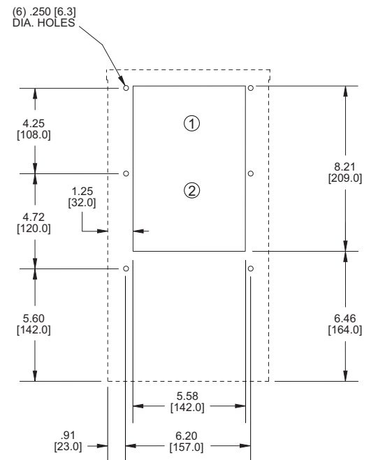
MOUNTING PLAN
