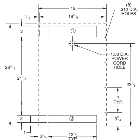
MOUNTING PLAN
