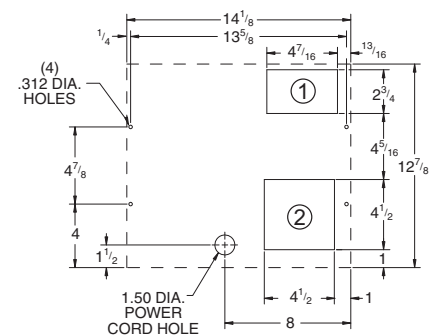
MOUNTING PLAN
