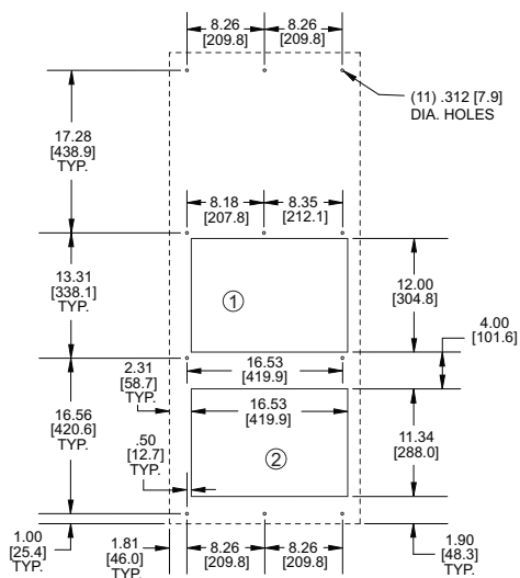
MOUNTING PLAN
