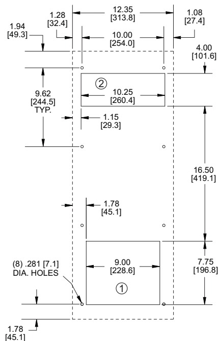
MOUNTING PLAN
