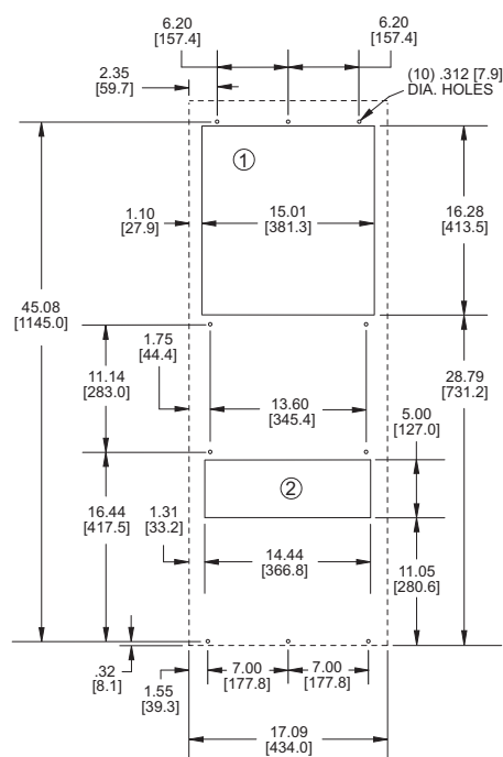
MOUNTING PLAN
