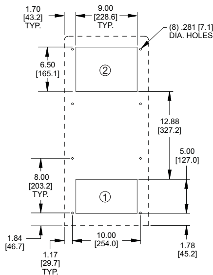
MOUNTING PLAN
