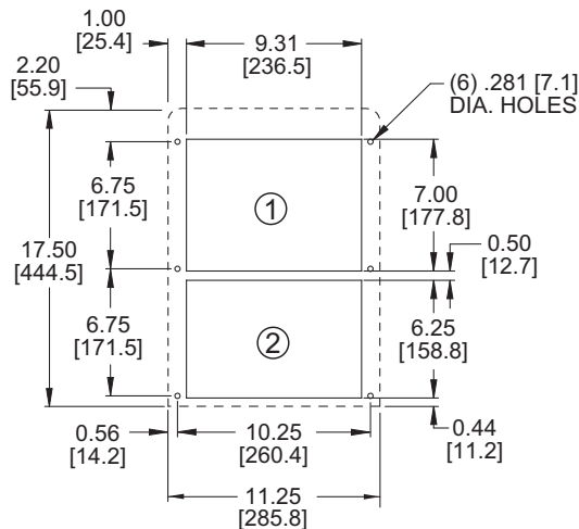
MOUNTING PLAN
