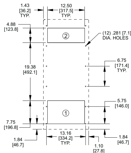
MOUNTING PLAN
