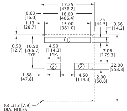
MOUNTING PLAN
