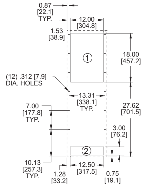
MOUNTING PLAN
