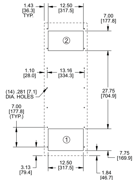
MOUNTING PLAN
