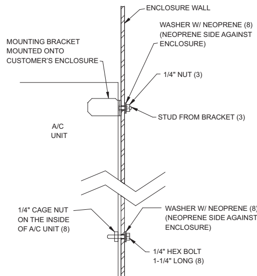
MOUNTING DRAWING
