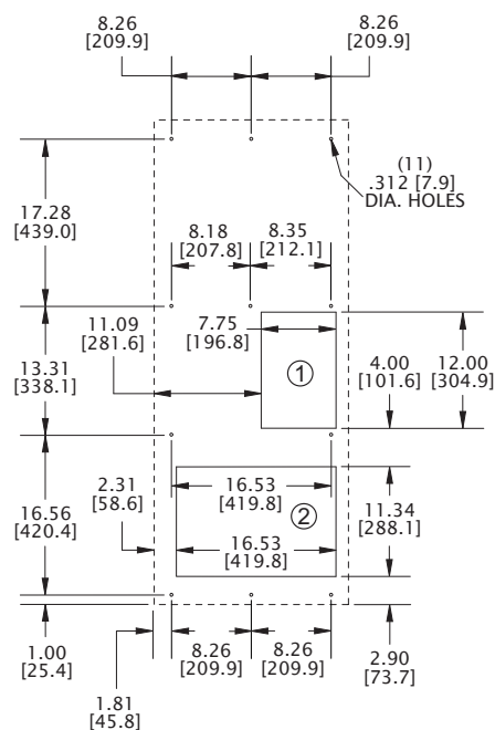
MOUNTING PLAN
