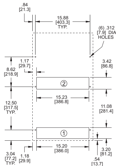
MOUNTING PLAN
