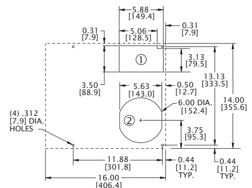
MOUNTING PLAN
