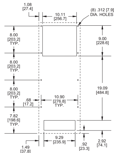
MOUNTING PLAN
