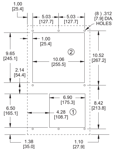
MOUNTING PLAN
