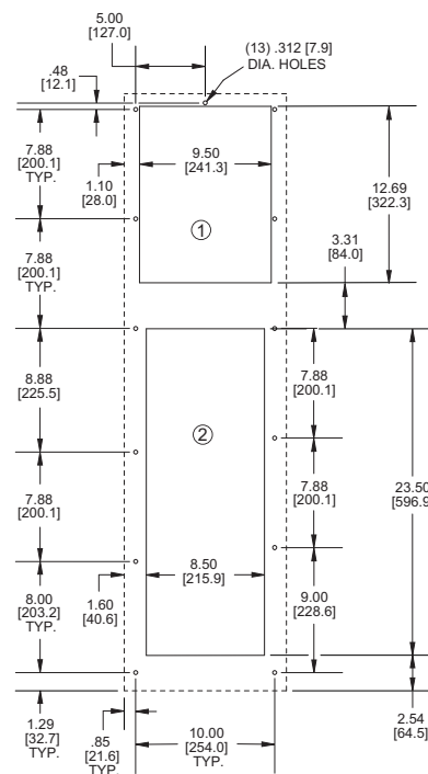
MOUNTING PLAN
