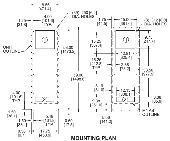
MOUNTING PLAN
