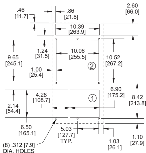
MOUNTING PLAN
