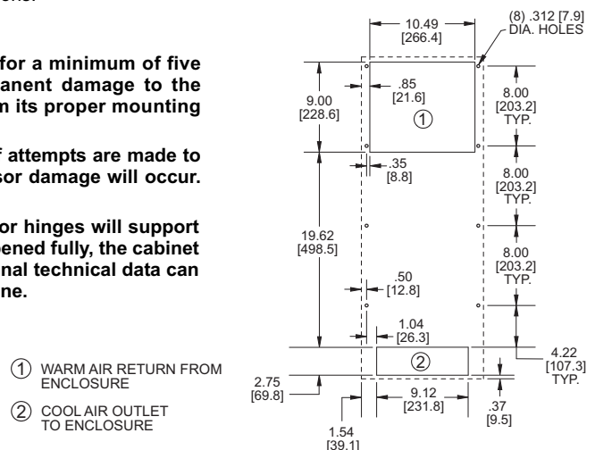
MOUNTING PLAN
