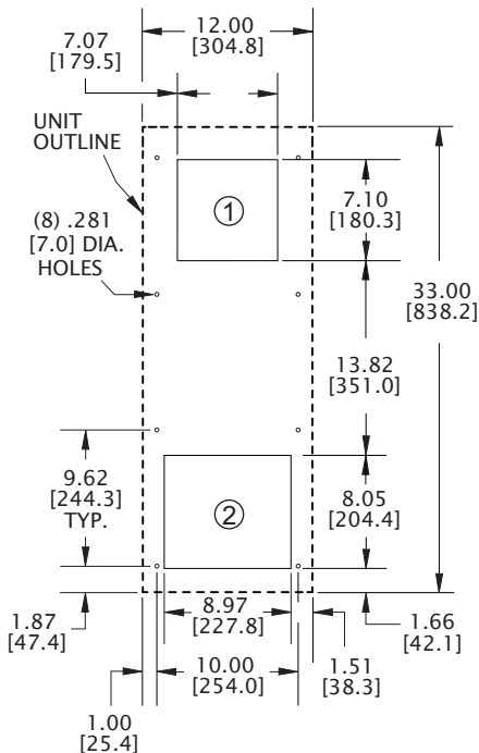
MOUNTING PLAN
