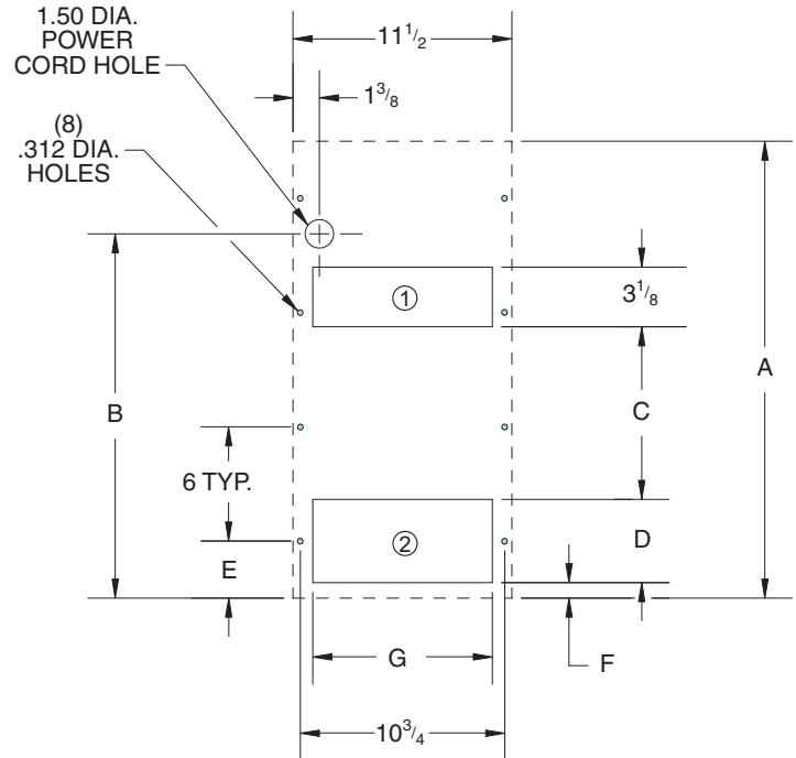
MOUNTING PLAN
