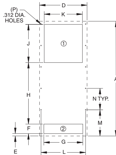
MOUNTING PLAN
