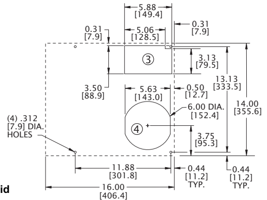
MOUNTING PLAN
