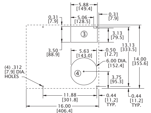
MOUNTING PLAN
