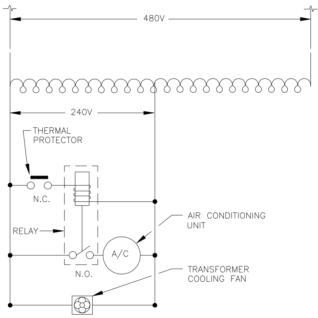
WIRING DIAGRAM
