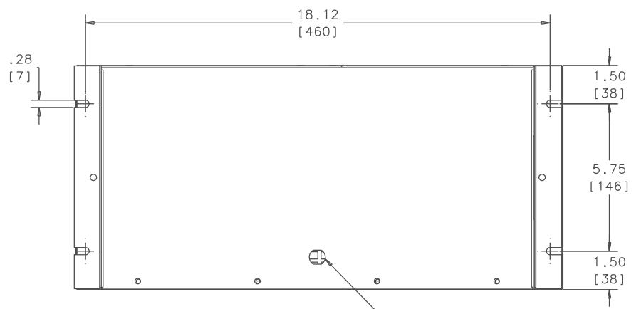
BACK VIEW 3 FOOT MIN CORD EXIT
