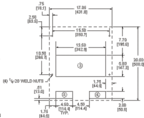
MOUNTING PLAN
