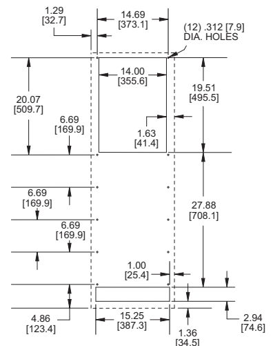
MOUNTING PLAN
