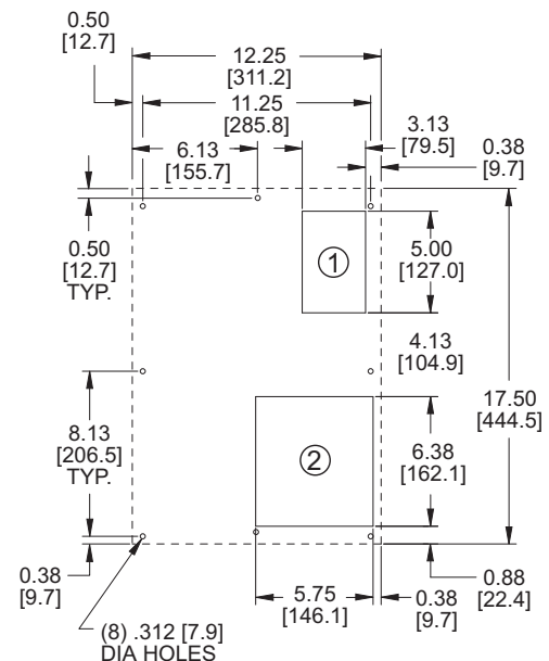
MOUNTING PLAN
