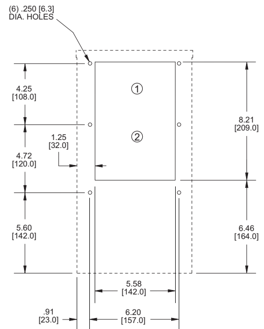
MOUNTING PLAN
