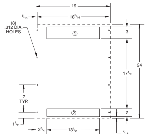
MOUNTING PLAN
