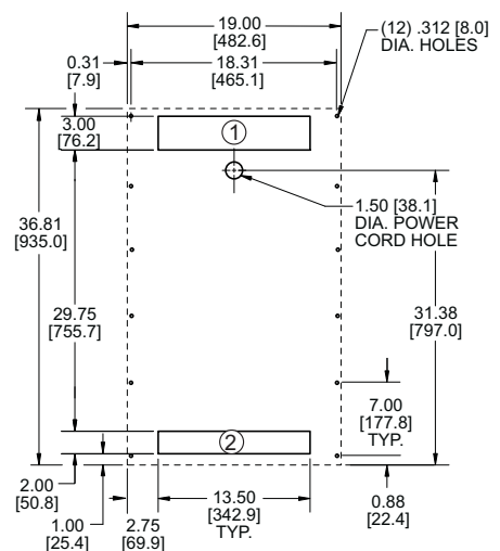
MOUNTING PLAN
