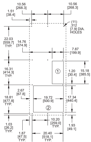
MOUNTING PLAN
