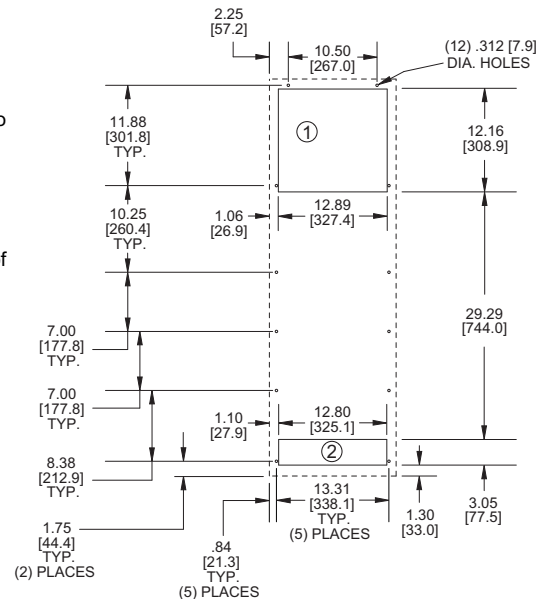
MOUNTING PLAN
