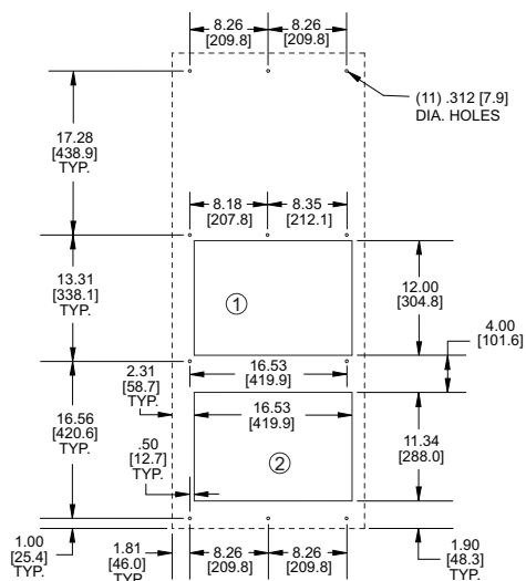
MOUNTING PLAN
