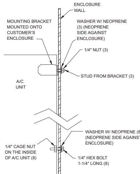
MOUNTING DRAWING
