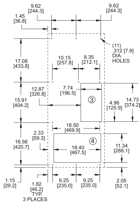
MOUNTING PLAN
