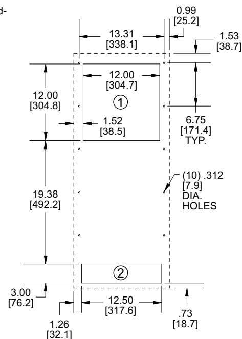
MOUNTING PLAN
