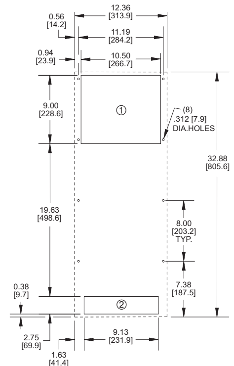
MOUNTING PLAN
