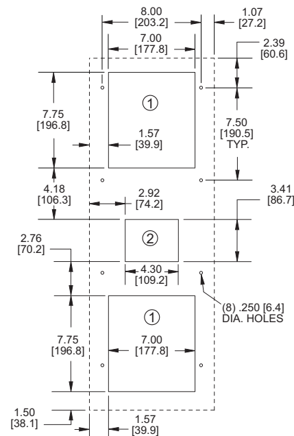
MOUNTING PLAN
