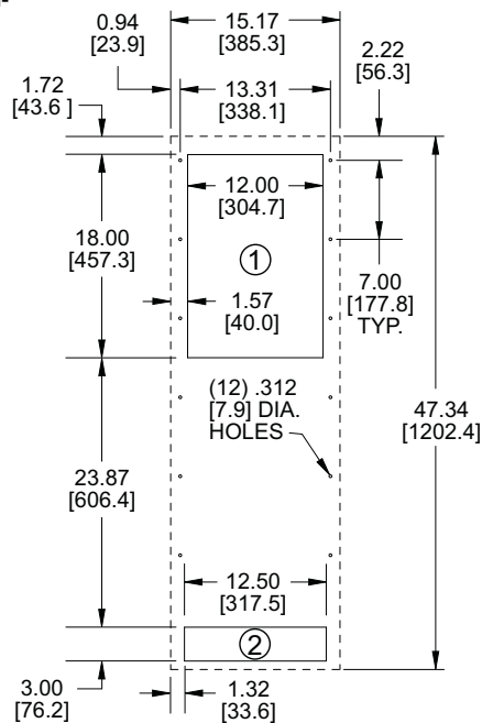
MOUNTING PLAN
