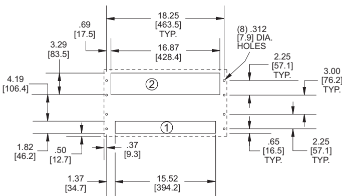
MOUNTING PLAN
