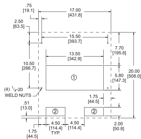
MOUNTING PLAN
