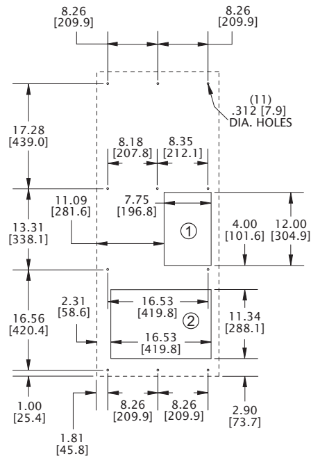
MOUNTING PLAN
