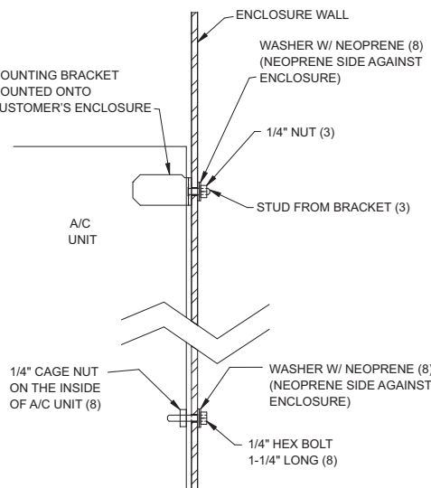
MOUNTING DRAWING
