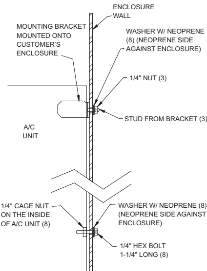
MOUNTING DRAWING
