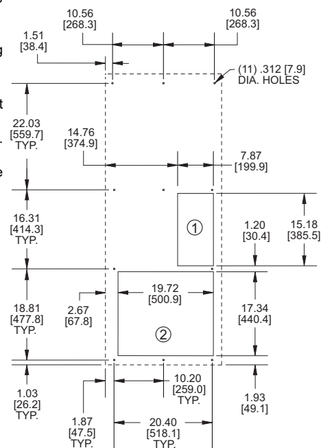
MOUNTING PLAN
