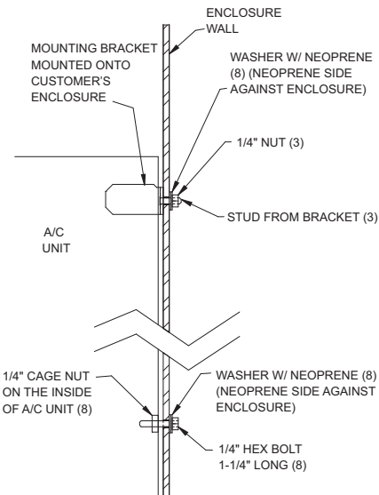
MOUNTING DRAWING
