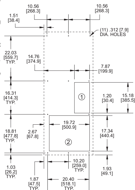
MOUNTING PLAN
