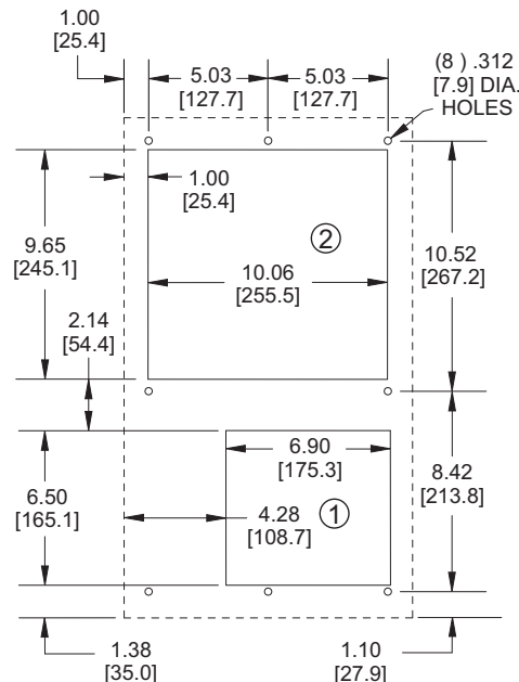
MOUNTING PLAN
