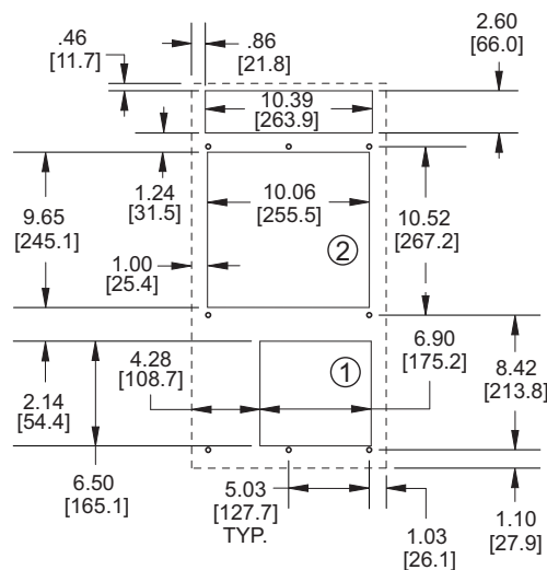
MOUNTING PLAN
