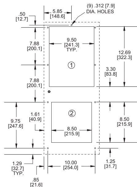
MOUNTING PLAN
